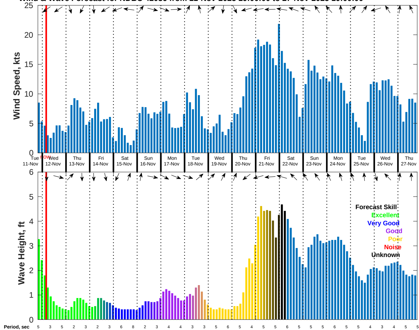
Wind & Wave Forecast for NDBC 42036 from 11-Nov-2025 19:00:00 to 27-Nov-2025 19:00:00
