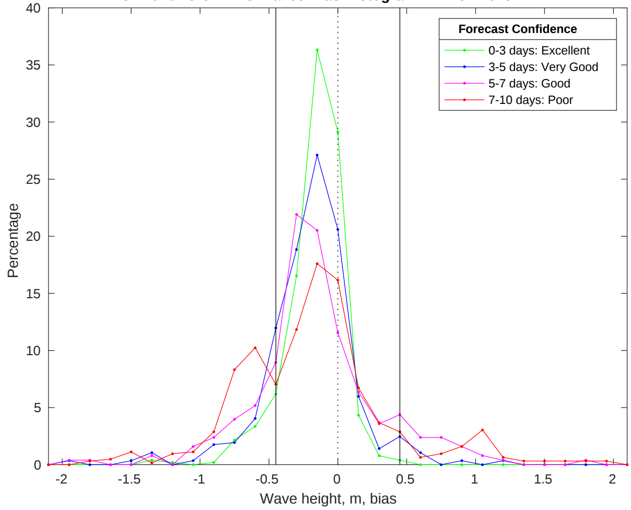
NDBC 42040 vs CMEMS Waves Bias Histogram: 12-Nov-2025
