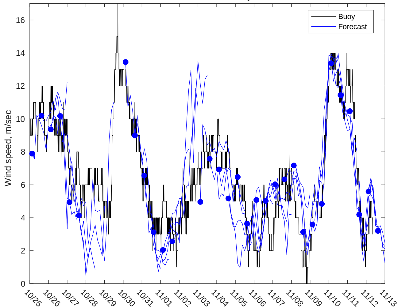
NDBC 42040 vs GFS Winds: 3 to 5 day forecast
