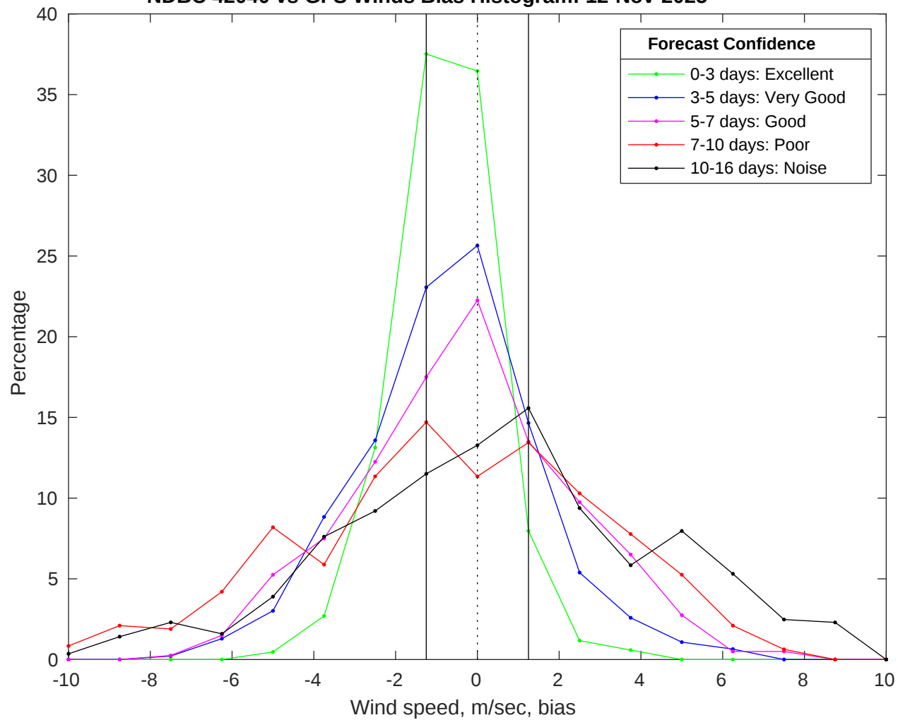
NDBC 42040 vs GFS Winds Bias Histogram: 12-Nov-2025
