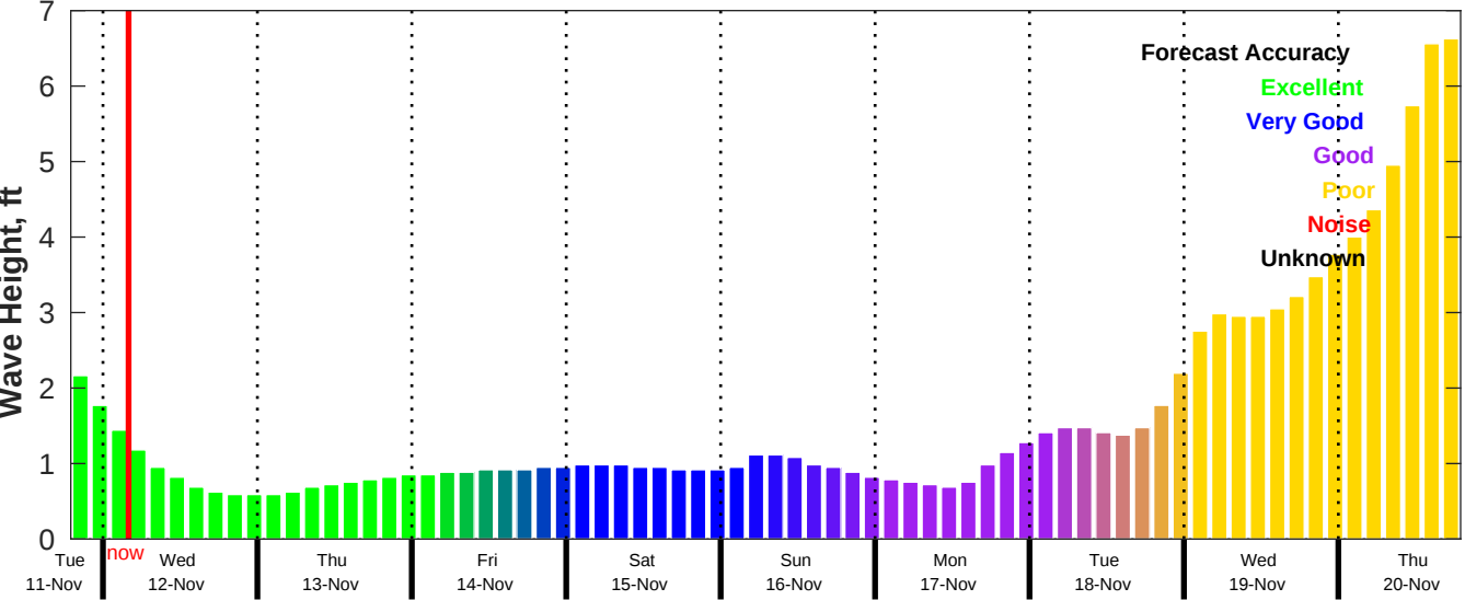
CMEMS Wave Forecast for NDBC 42040 from 11-Nov-2025 19:00:00 to 20-Nov-2025 19:00:00
