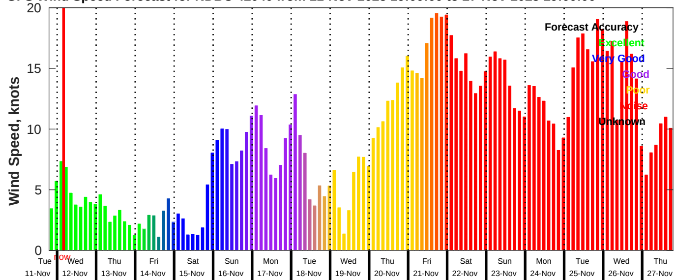
GFS Wind Speed Forecast for NDBC 42040 from 11-Nov-2025 19:00:00 to 27-Nov-2025 19:00:00
