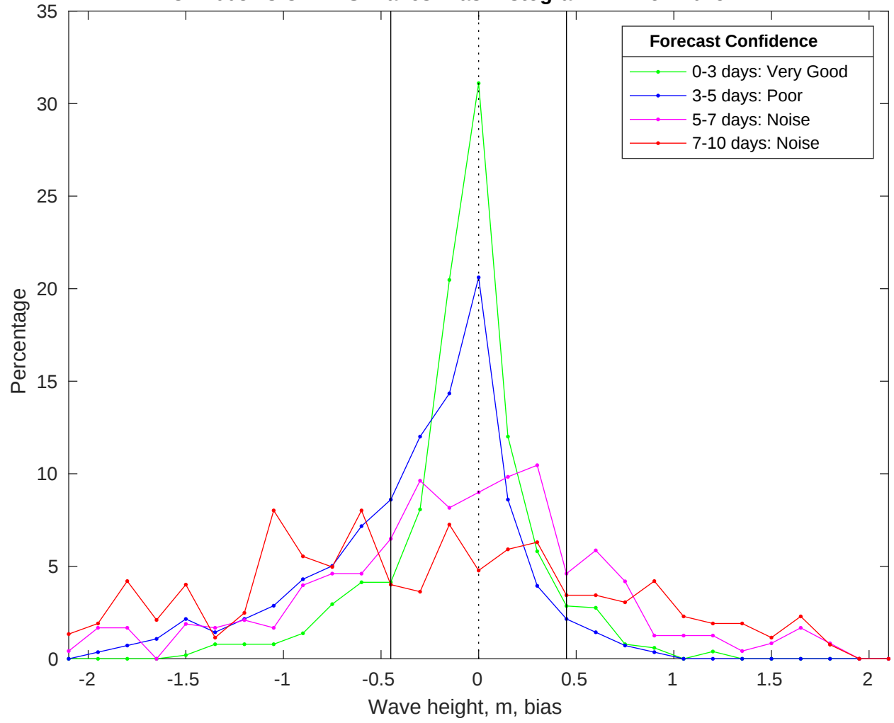
NDBC 44008 vs CMEMS Waves Bias Histogram: 12-Nov-2025
