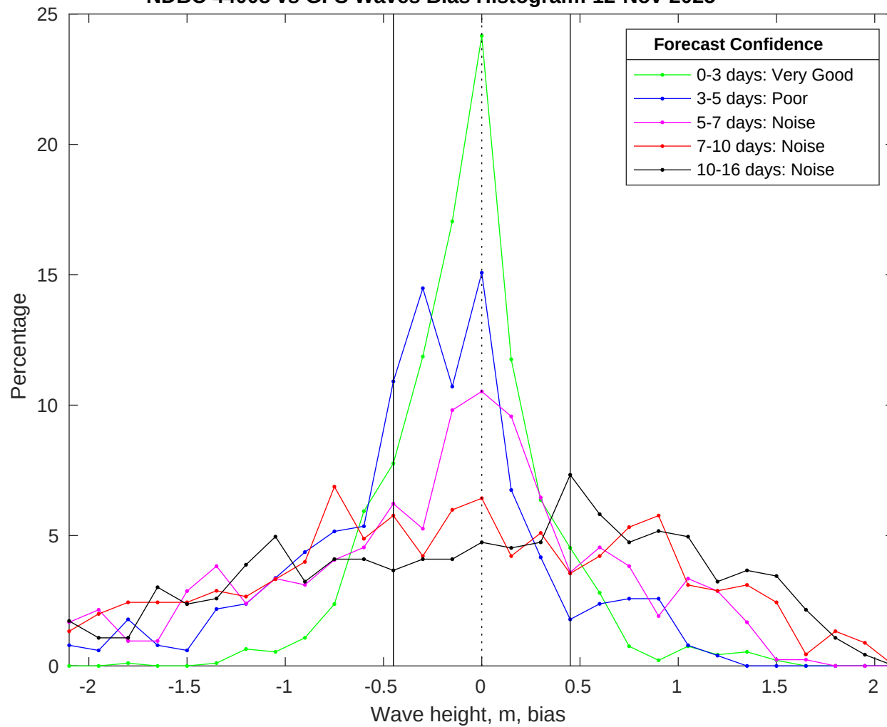
NDBC 44008 vs GFS Waves Bias Histogram: 12-Nov-2025
