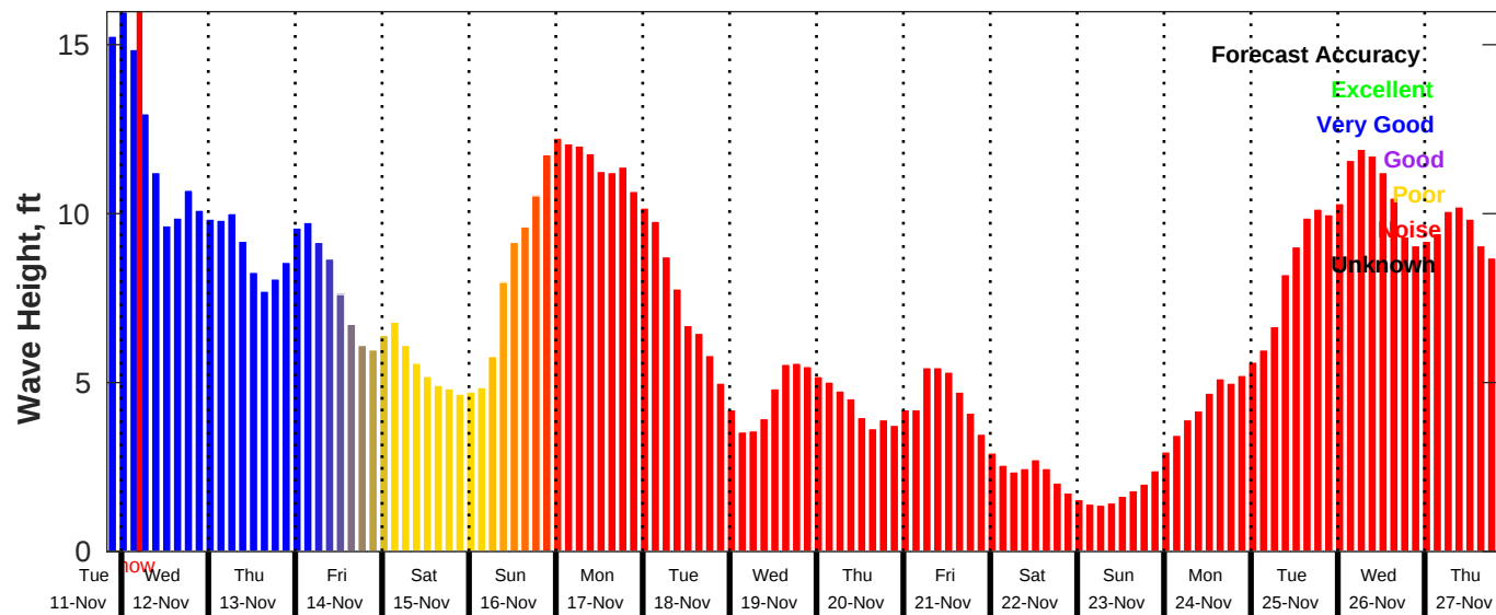
GFS Wave Forecast for NDBC 44008 from 11-Nov-2025 20:00:00 to 27-Nov-2025 20:00:00
