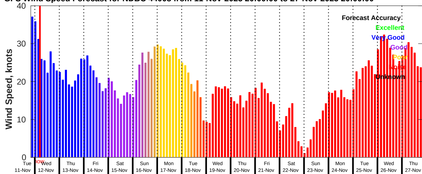
GFS Wind Speed Forecast for NDBC 44008 from 11-Nov-2025 20:00:00 to 27-Nov-2025 20:00:00
