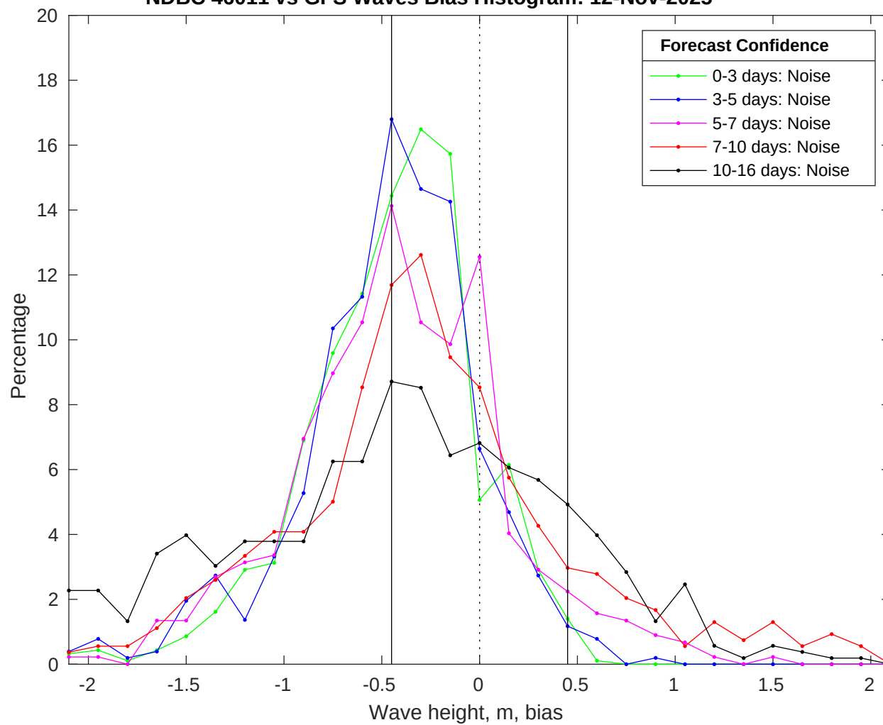
NDBC 46011 vs GFS Waves Bias Histogram: 12-Nov-2025
