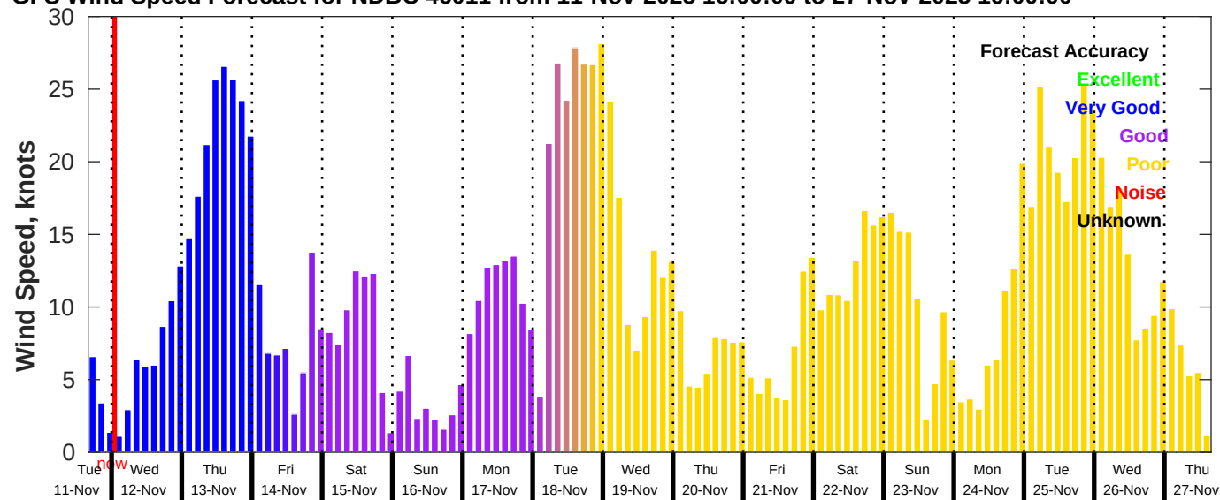
GFS Wind Speed Forecast for NDBC 46011 from 11-Nov-2025 16:00:00 to 27-Nov-2025 16:00:00
