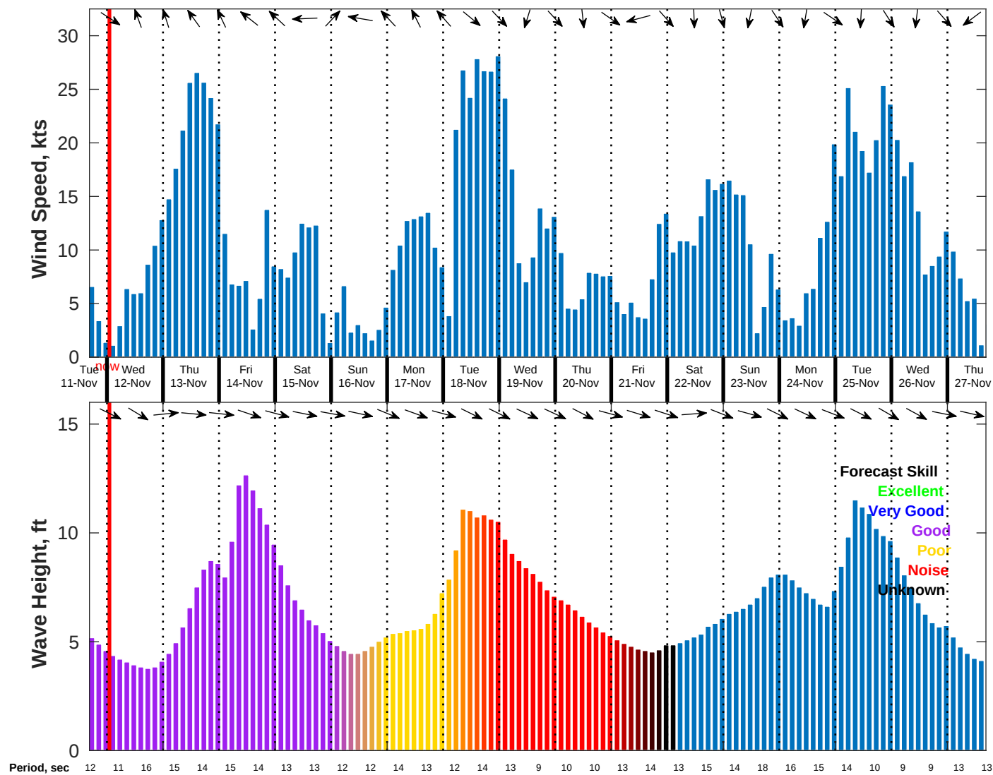
Wind & Wave Forecast for NDBC 46011 from 11-Nov-2025 16:00:00 to 27-Nov-2025 16:00:00
