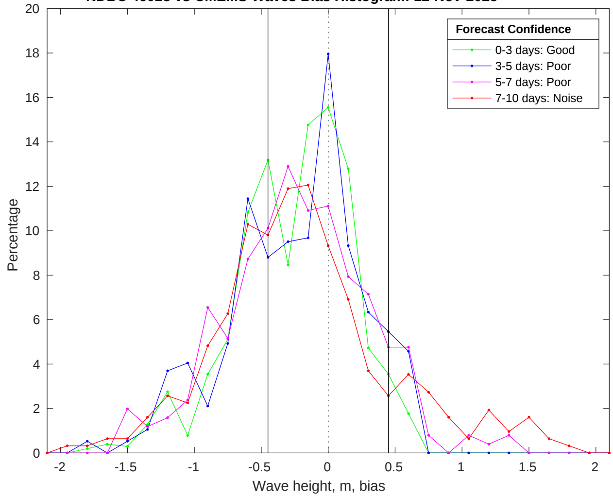
NDBC 46028 vs CMEMS Waves Bias Histogram: 12-Nov-2025
