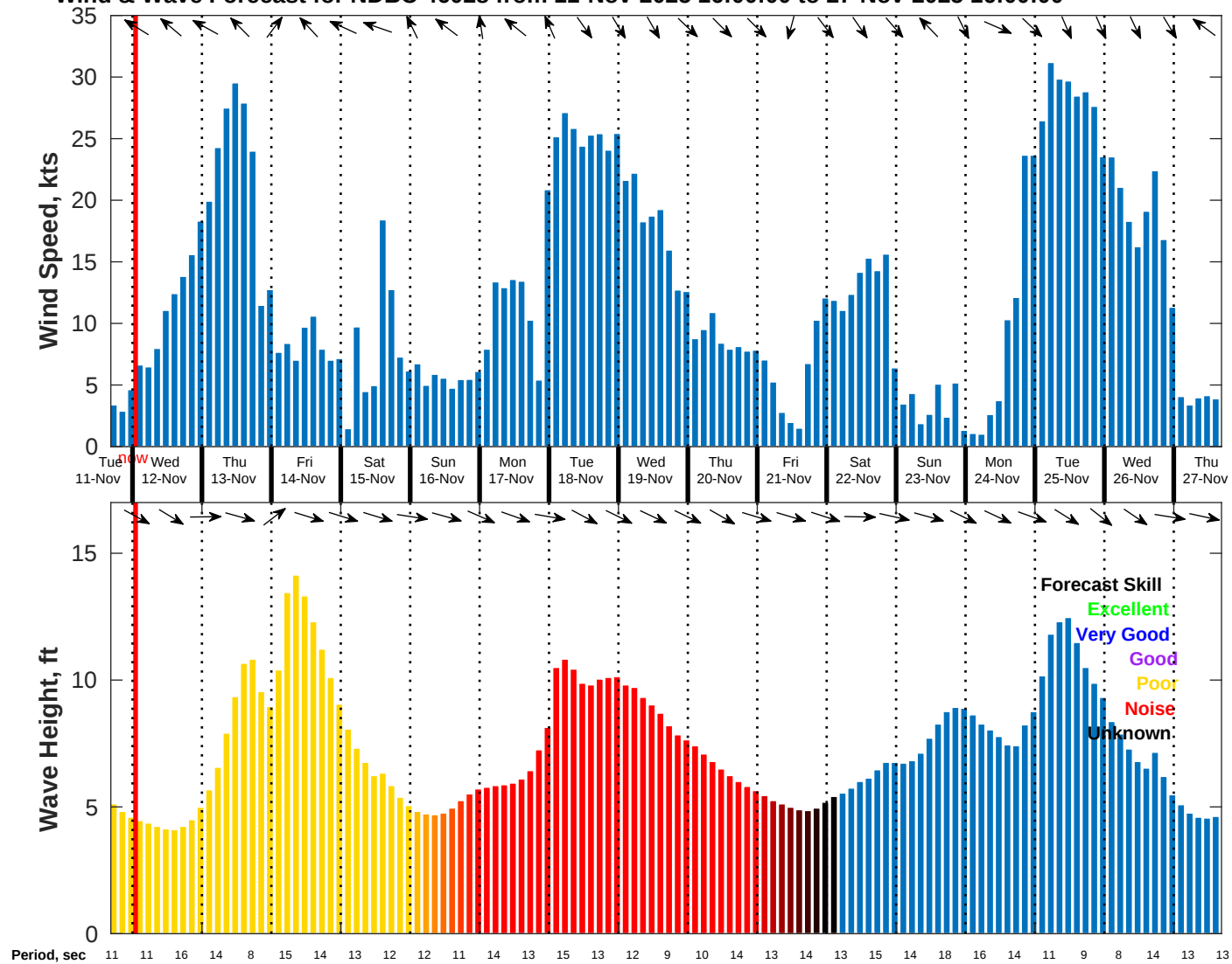
Wind & Wave Forecast for NDBC 46028 from 11-Nov-2025 16:00:00 to 27-Nov-2025 16:00:00
