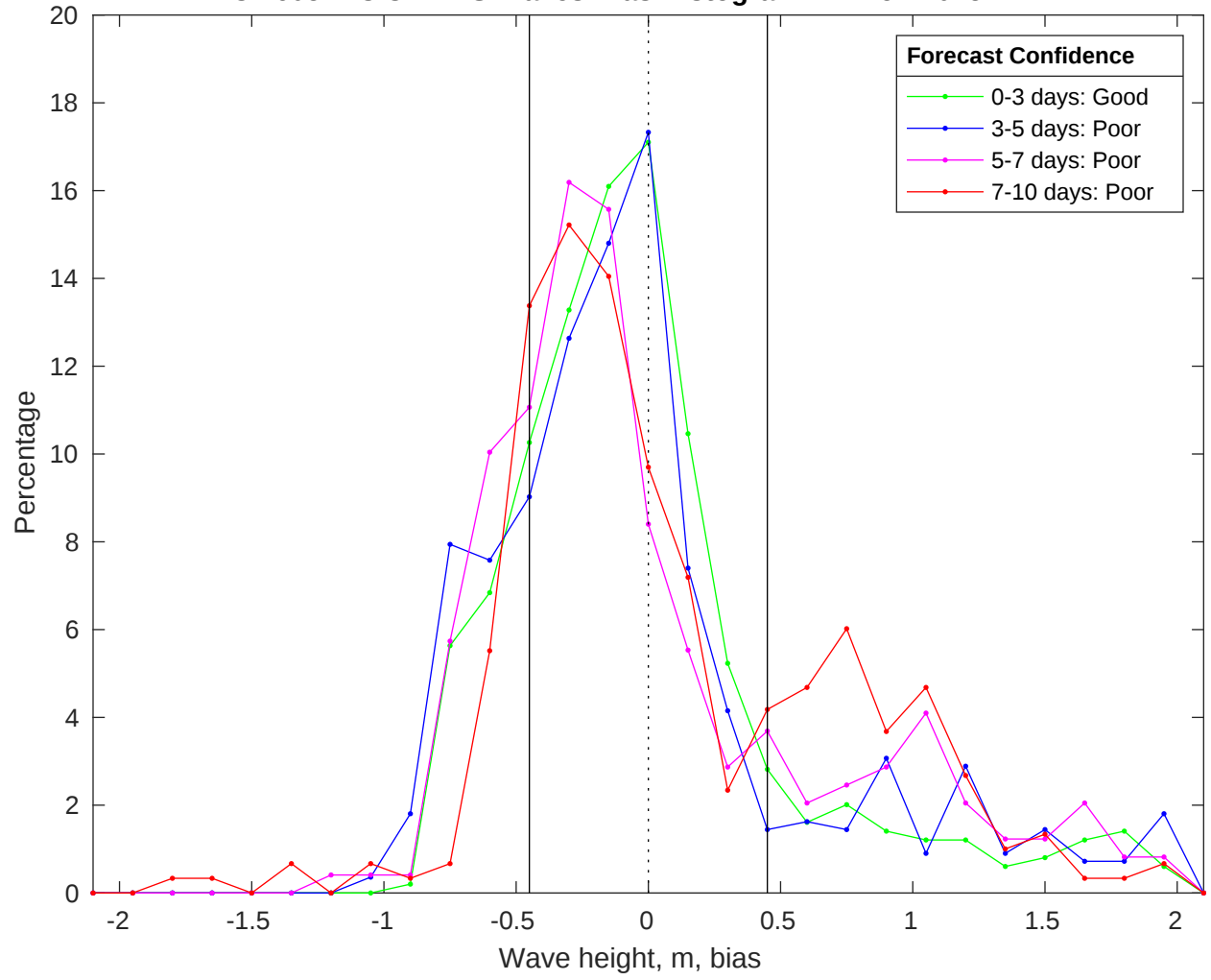
NDBC 46054 vs CMEMS Waves Bias Histogram: 11-Nov-2025
