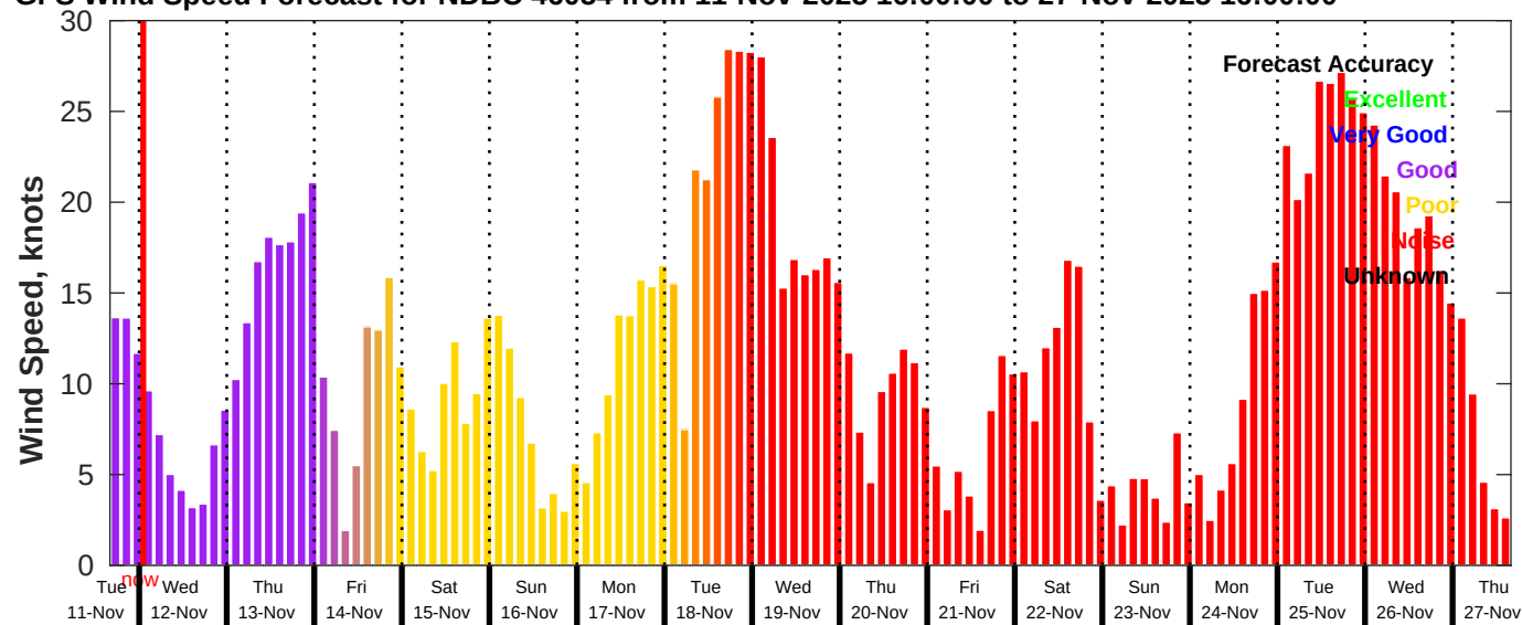
GFS Wind Speed Forecast for NDBC 46054 from 11-Nov-2025 16:00:00 to 27-Nov-2025 16:00:00
