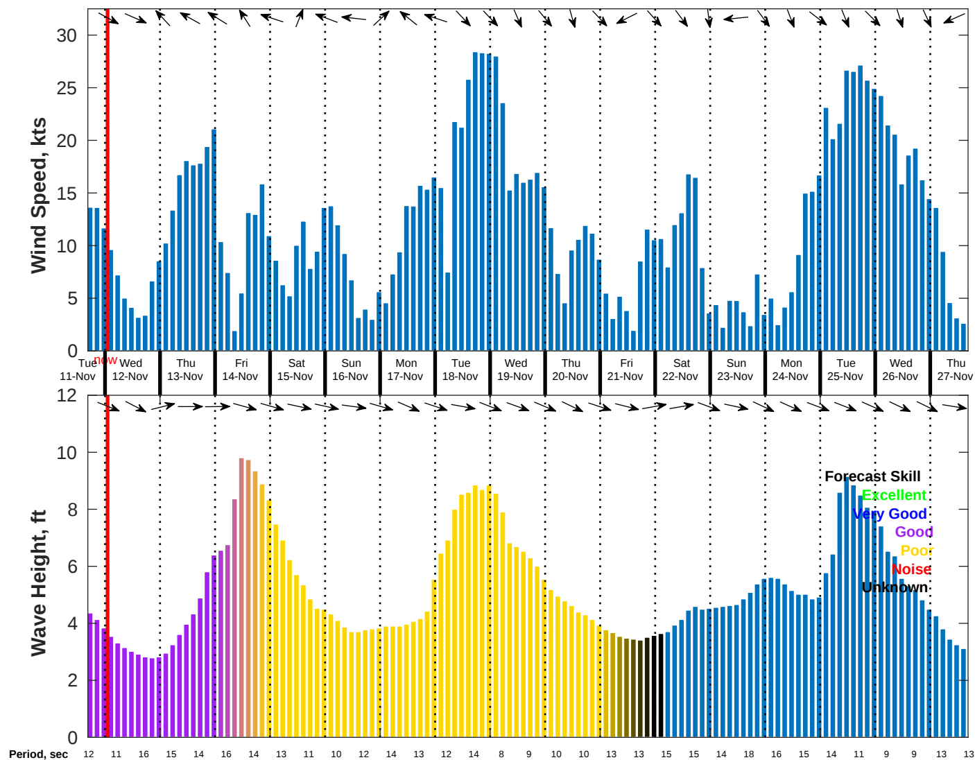
Wind & Wave Forecast for NDBC 46054 from 11-Nov-2025 16:00:00 to 27-Nov-2025 16:00:00
