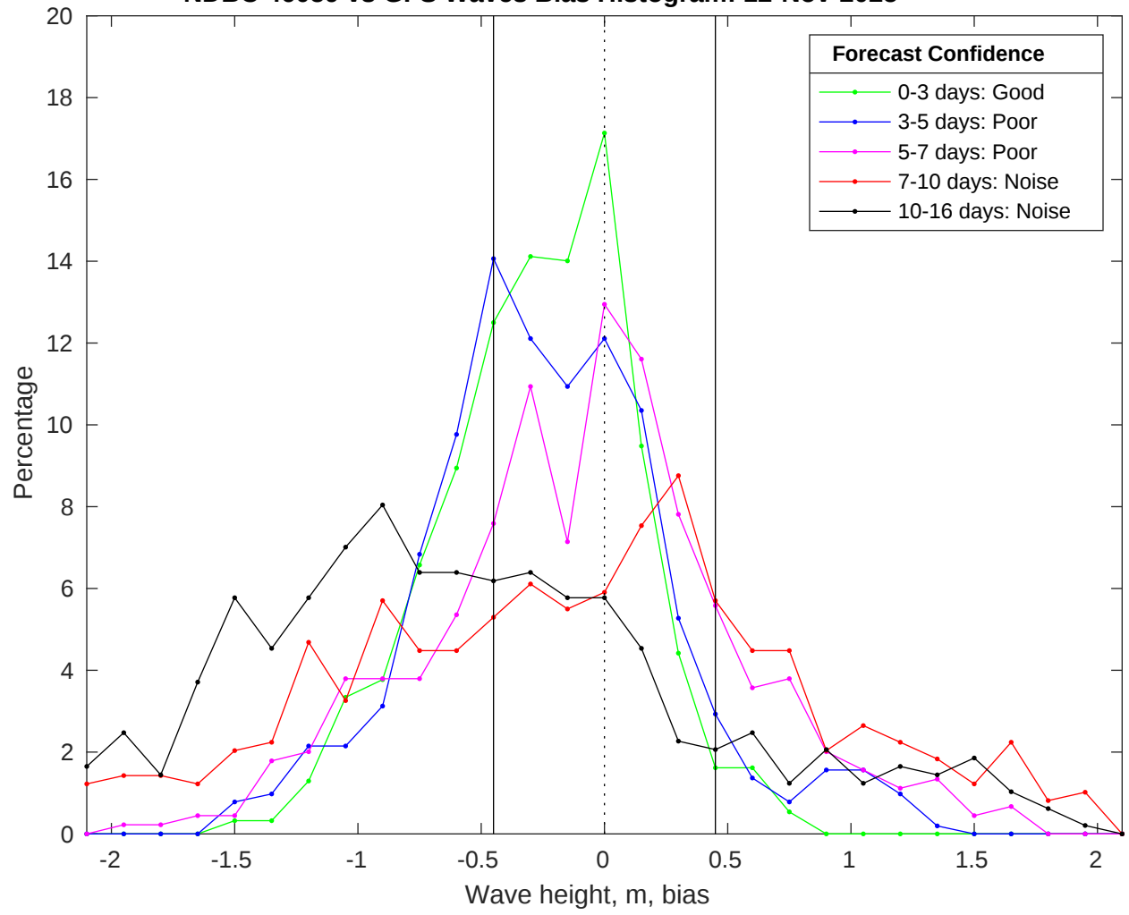
NDBC 46059 vs GFS Waves Bias Histogram: 12-Nov-2025
