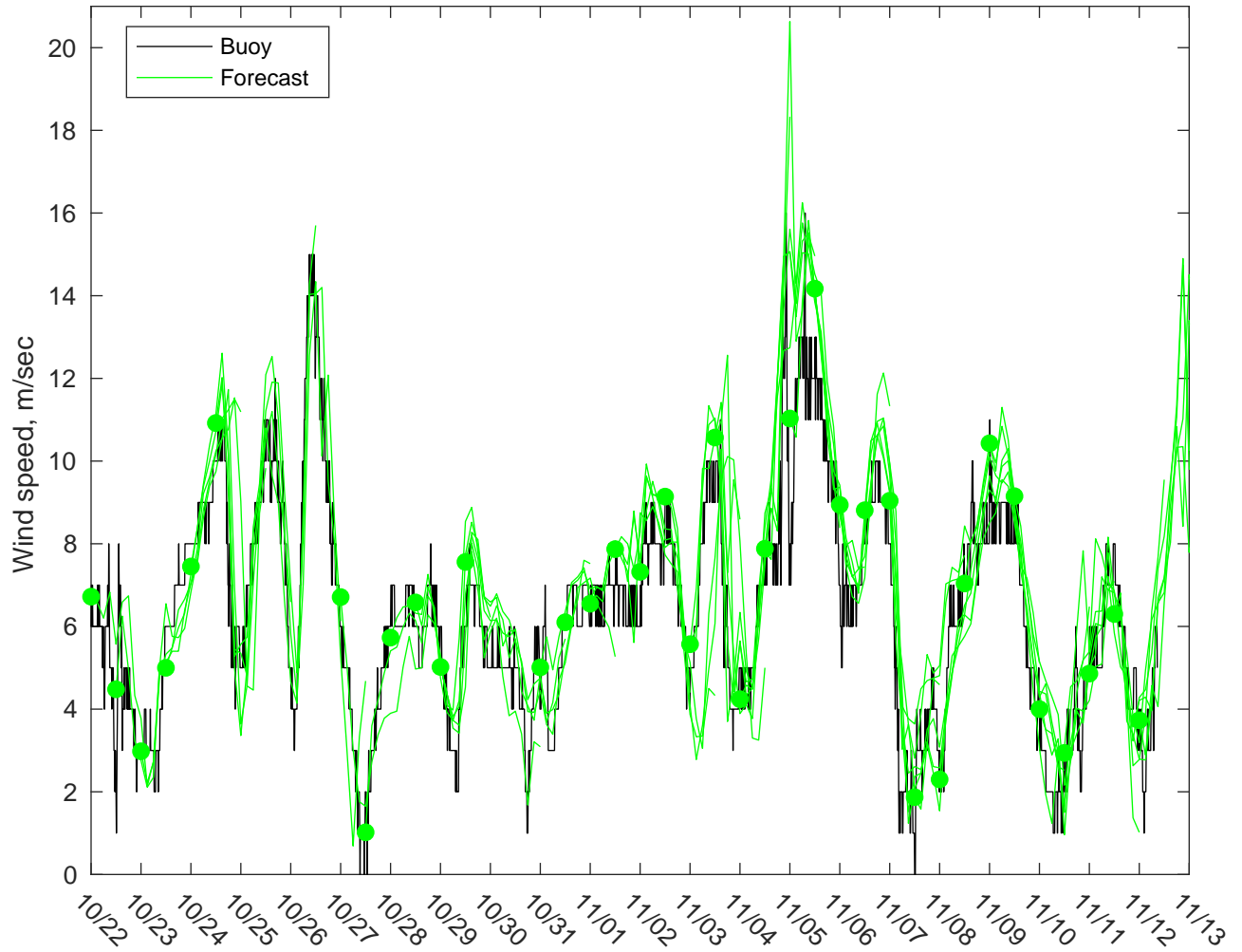
NDBC 46059 vs GFS Winds: 0 to 3 day forecast
