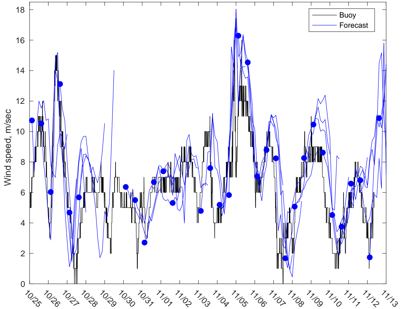
NDBC 46059 vs GFS Winds: 3 to 5 day forecast
