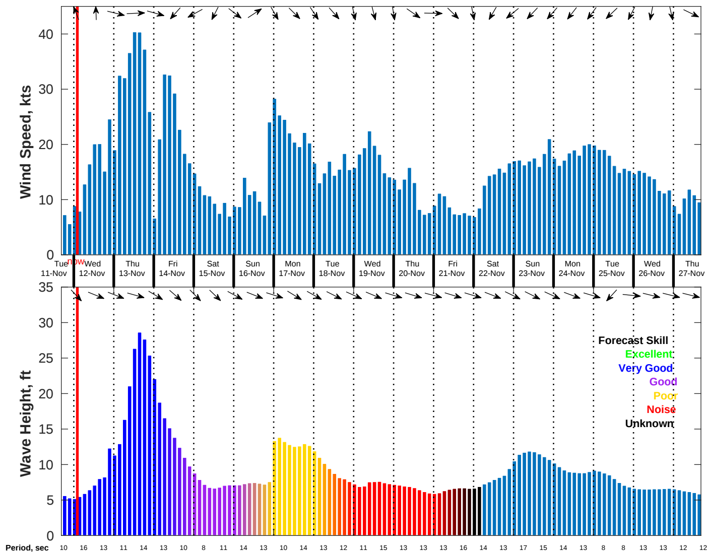
Wind & Wave Forecast for NDBC 46059 from 11-Nov-2025 17:00:00 to 27-Nov-2025 17:00:00
