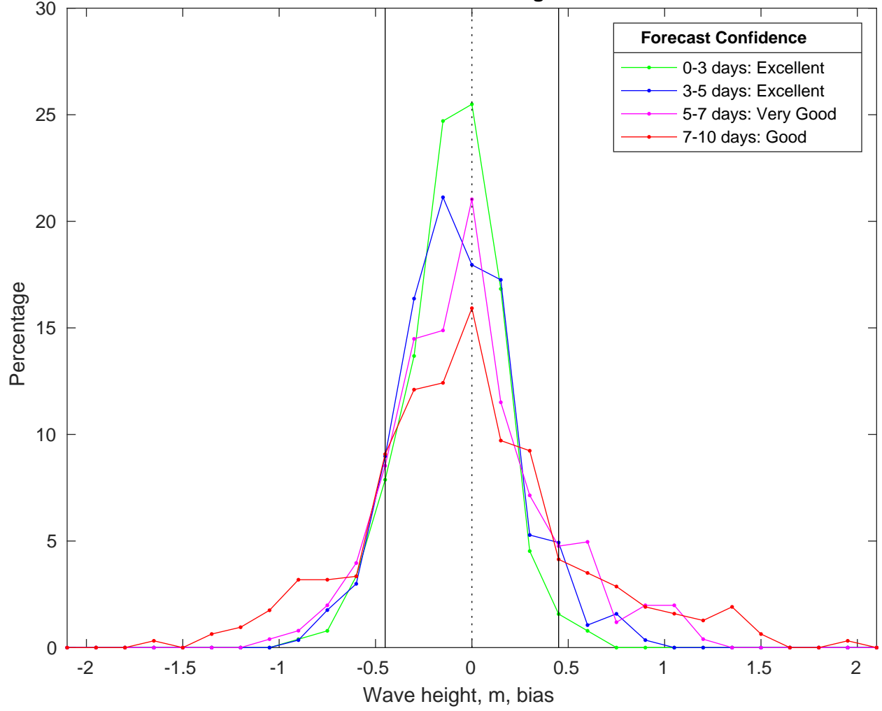
NDBC 46069 vs CMEMS Waves Bias Histogram: 12-Nov-2025
