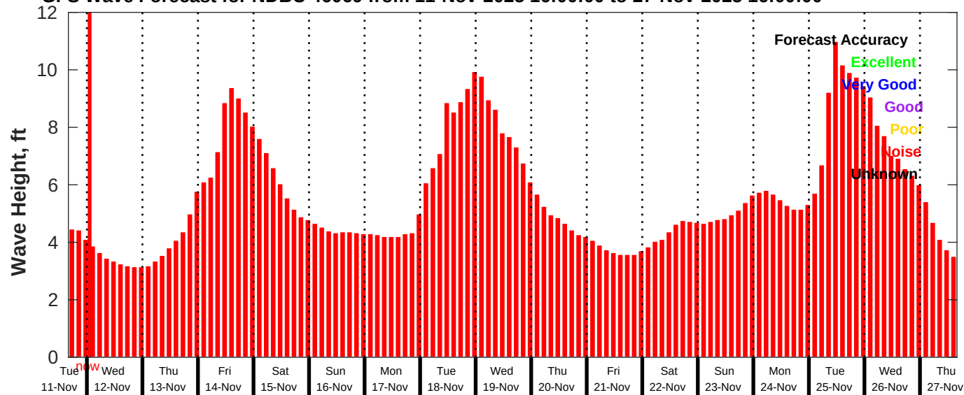
GFS Wave Forecast for NDBC 46069 from 11-Nov-2025 16:00:00 to 27-Nov-2025 16:00:00
