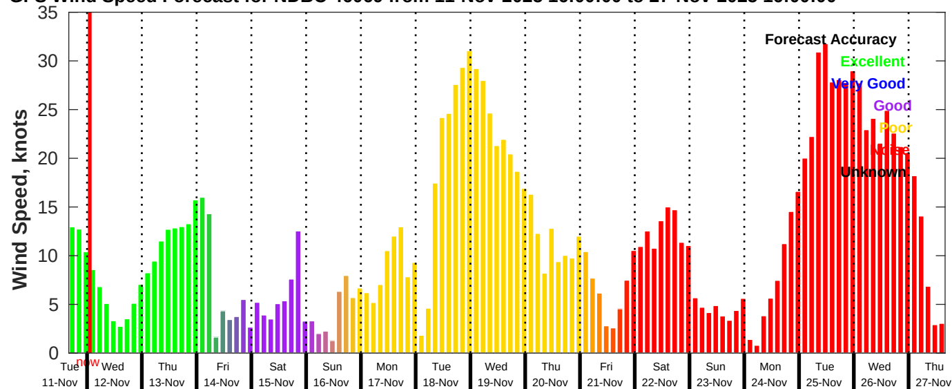
GFS Wind Speed Forecast for NDBC 46069 from 11-Nov-2025 16:00:00 to 27-Nov-2025 16:00:00
