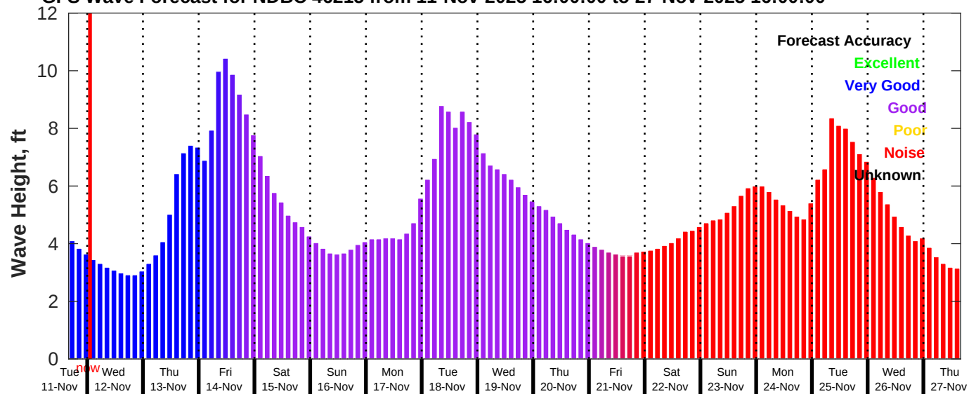
GFS Wave Forecast for NDBC 46215 from 11-Nov-2025 16:00:00 to 27-Nov-2025 16:00:00
