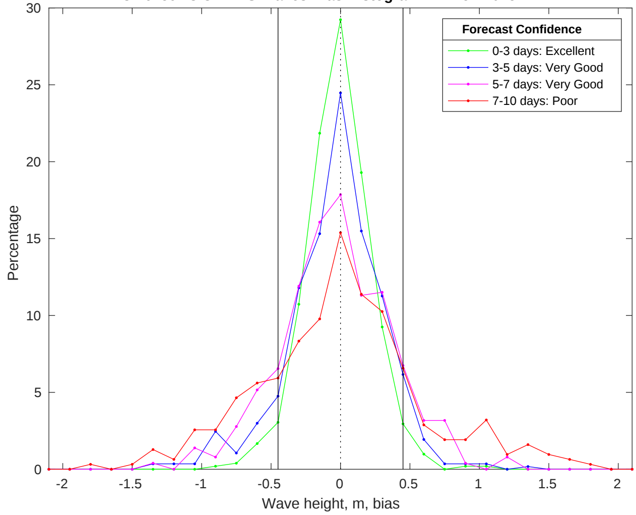
NDBC 46259 vs CMEMS Waves Bias Histogram: 12-Nov-2025
