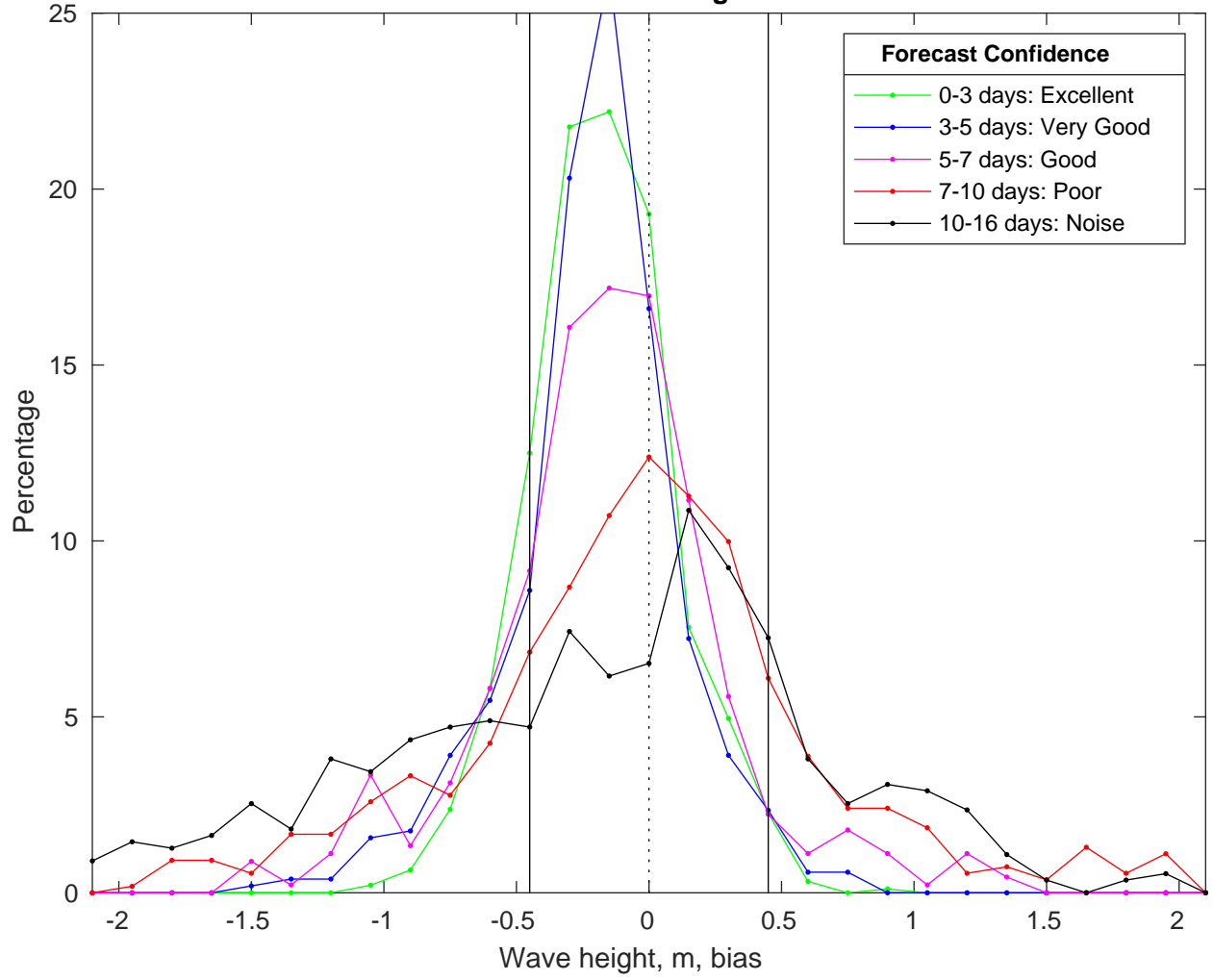
NDBC 46259 vs GFS Waves Bias Histogram: 12-Nov-2025
