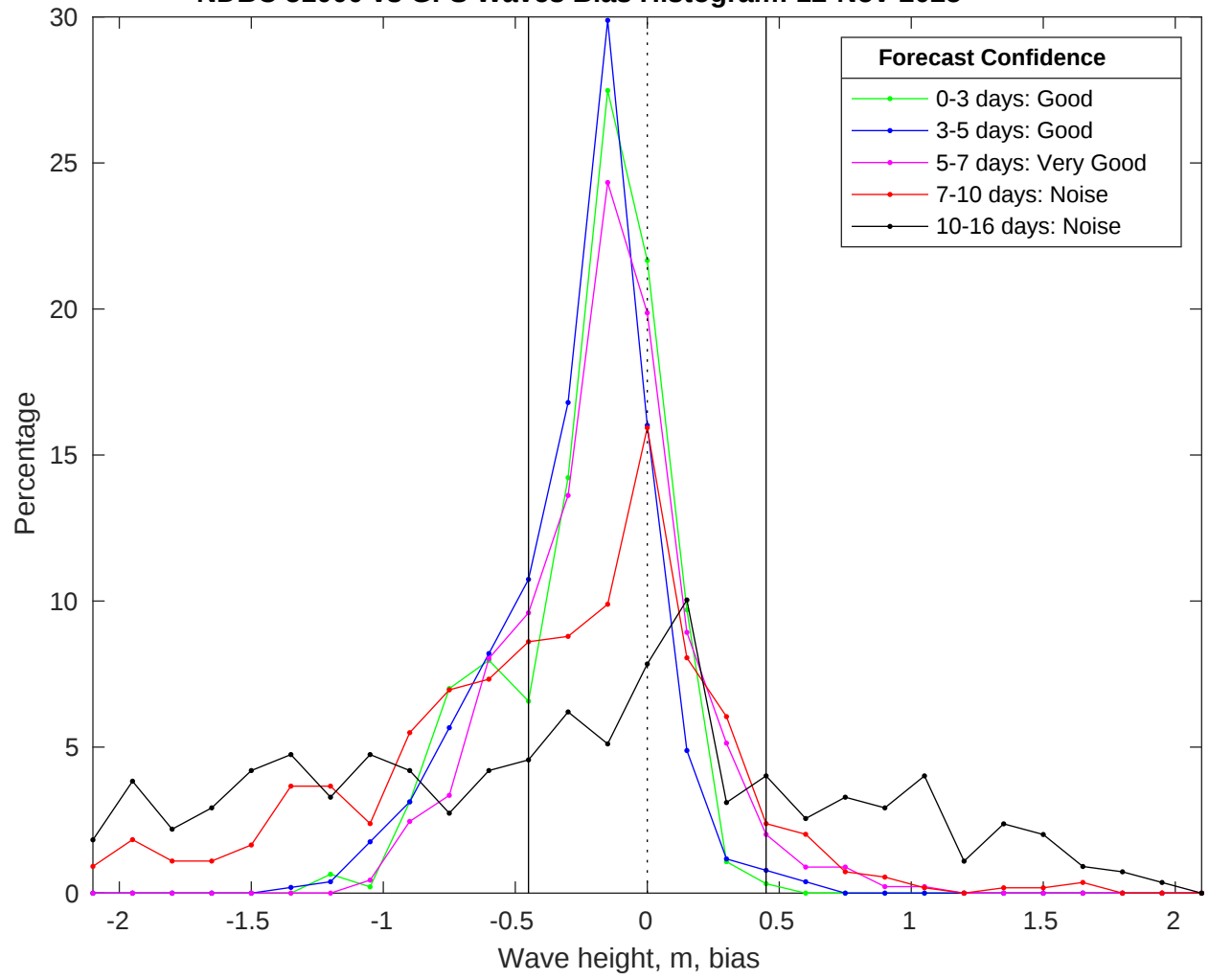
NDBC 51000 vs GFS Waves Bias Histogram: 12-Nov-2025
