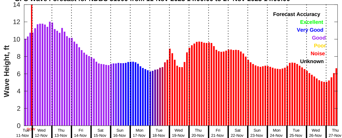
GFS Wave Forecast for NDBC 51000 from 11-Nov-2025 14:00:00 to 27-Nov-2025 14:00:00
