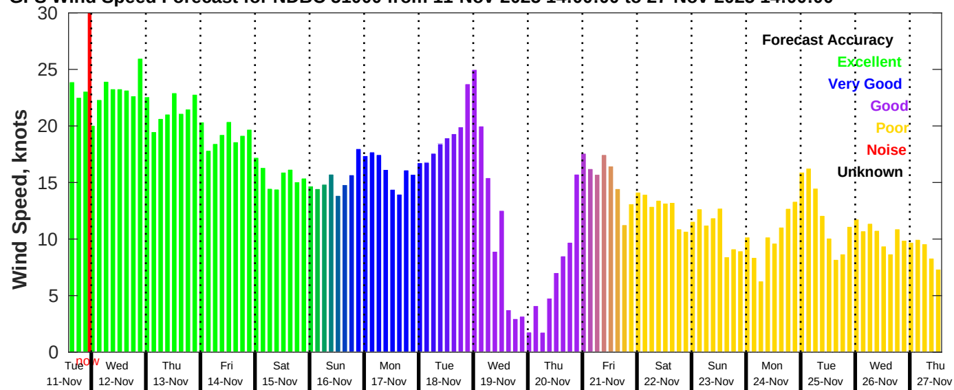
GFS Wind Speed Forecast for NDBC 51000 from 11-Nov-2025 14:00:00 to 27-Nov-2025 14:00:00
