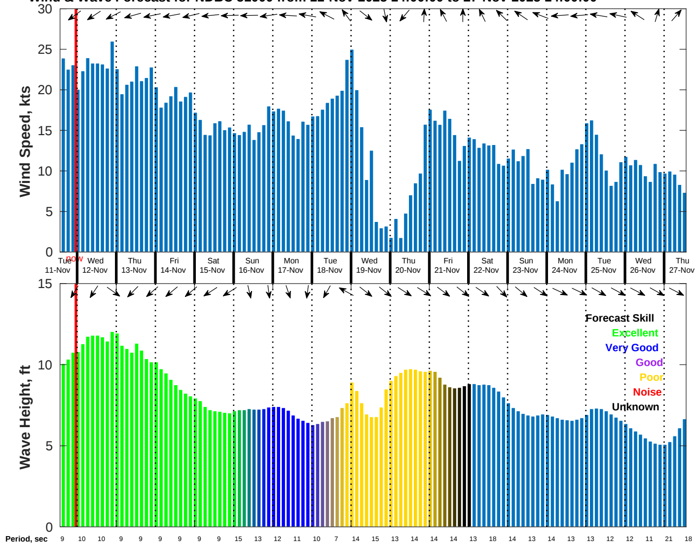
Wind & Wave Forecast for NDBC 51000 from 11-Nov-2025 14:00:00 to 27-Nov-2025 14:00:00
