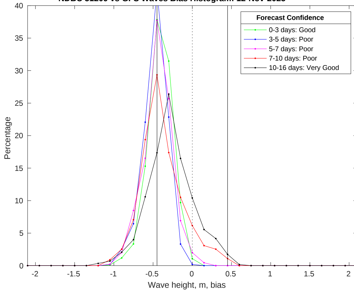
NDBC 51209 vs GFS Waves Bias Histogram: 12-Nov-2025
