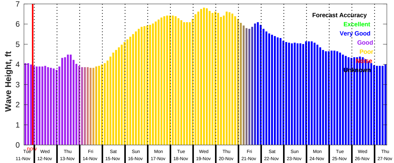
GFS Wave Forecast for NDBC 51209 from 11-Nov-2025 13:00:00 to 27-Nov-2025 13:00:00
