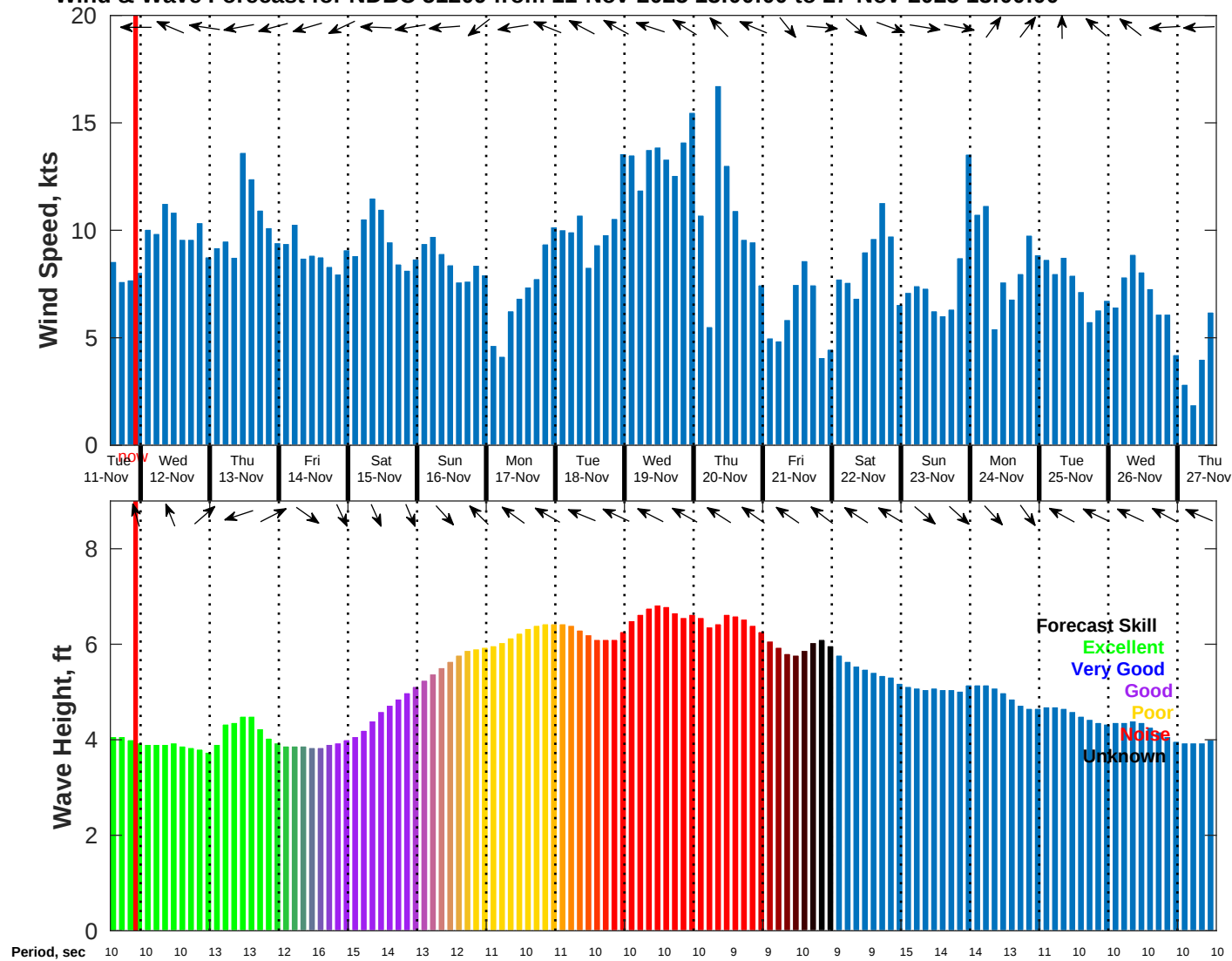
Wind & Wave Forecast for NDBC 51209 from 11-Nov-2025 13:00:00 to 27-Nov-2025 13:00:00
