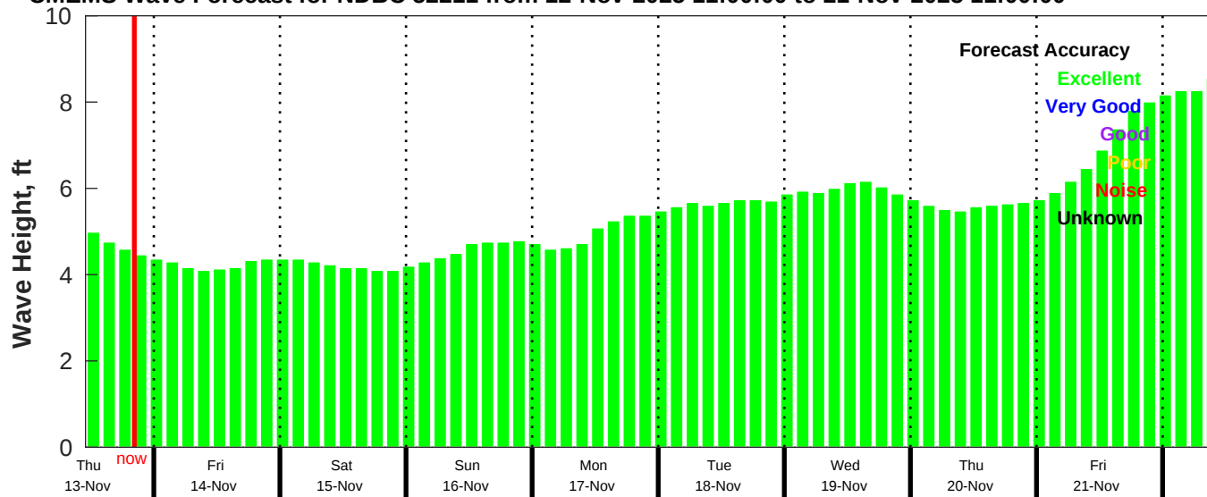
CMEMS Wave Forecast for NDBC 52211 from 12-Nov-2025 11:00:00 to 21-Nov-2025 11:00:00
