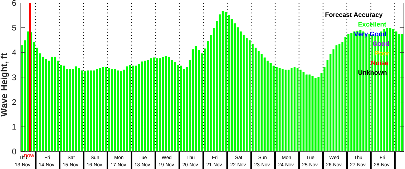
GFS Wave Forecast for NDBC 52212 from 12-Nov-2025 09:00:00 to 28-Nov-2025 09:00:00
