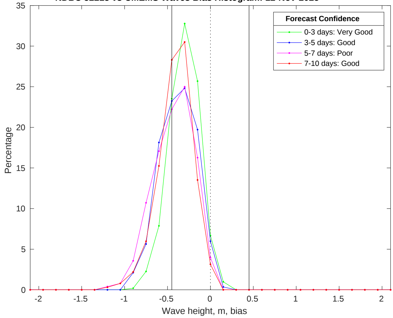
NDBC 52213 vs CMEMS Waves Bias Histogram: 12-Nov-2025
