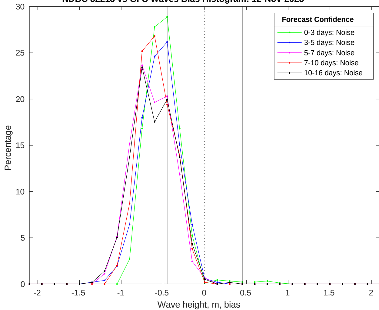
NDBC 52213 vs GFS Waves Bias Histogram: 12-Nov-2025
