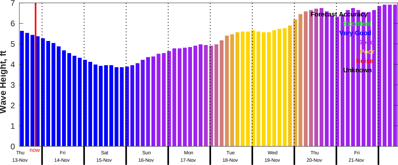
CMEMS Wave Forecast for NDBC 52213 from 12-Nov-2025 11:00:00 to 21-Nov-2025 11:00:00
