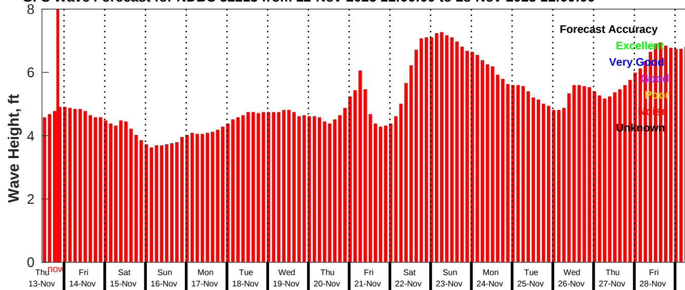
GFS Wave Forecast for NDBC 52213 from 12-Nov-2025 11:00:00 to 28-Nov-2025 11:00:00
