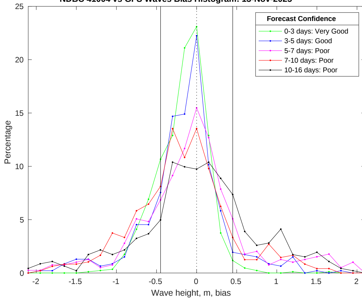
NDBC 41004 vs GFS Waves Bias Histogram: 13-Nov-2025
