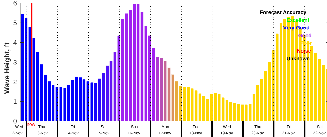
CMEMS Wave Forecast for NDBC 41004 from 12-Nov-2025 19:00:00 to 22-Nov-2025 19:00:00
