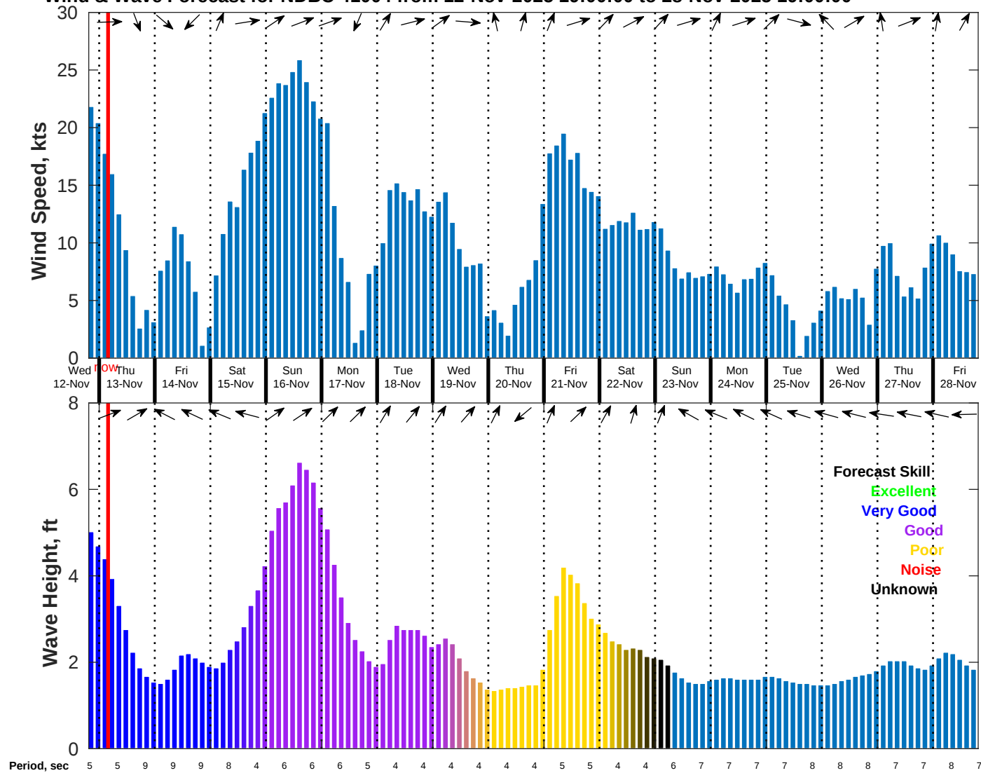
Wind & Wave Forecast for NDBC 41004 from 12-Nov-2025 19:00:00 to 28-Nov-2025 19:00:00
