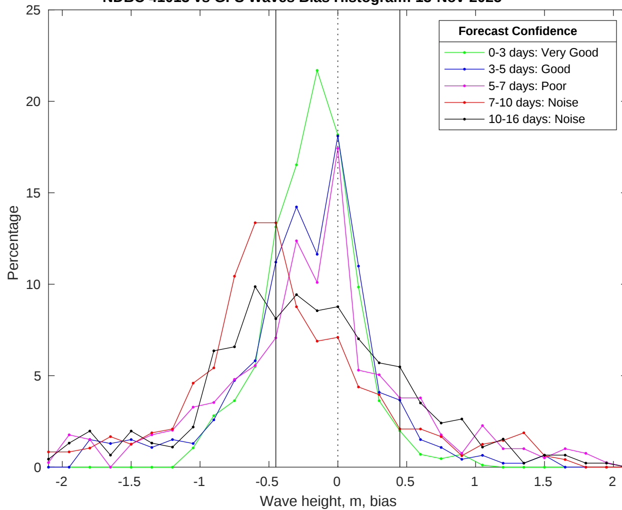
NDBC 41013 vs GFS Waves Bias Histogram: 13-Nov-2025
