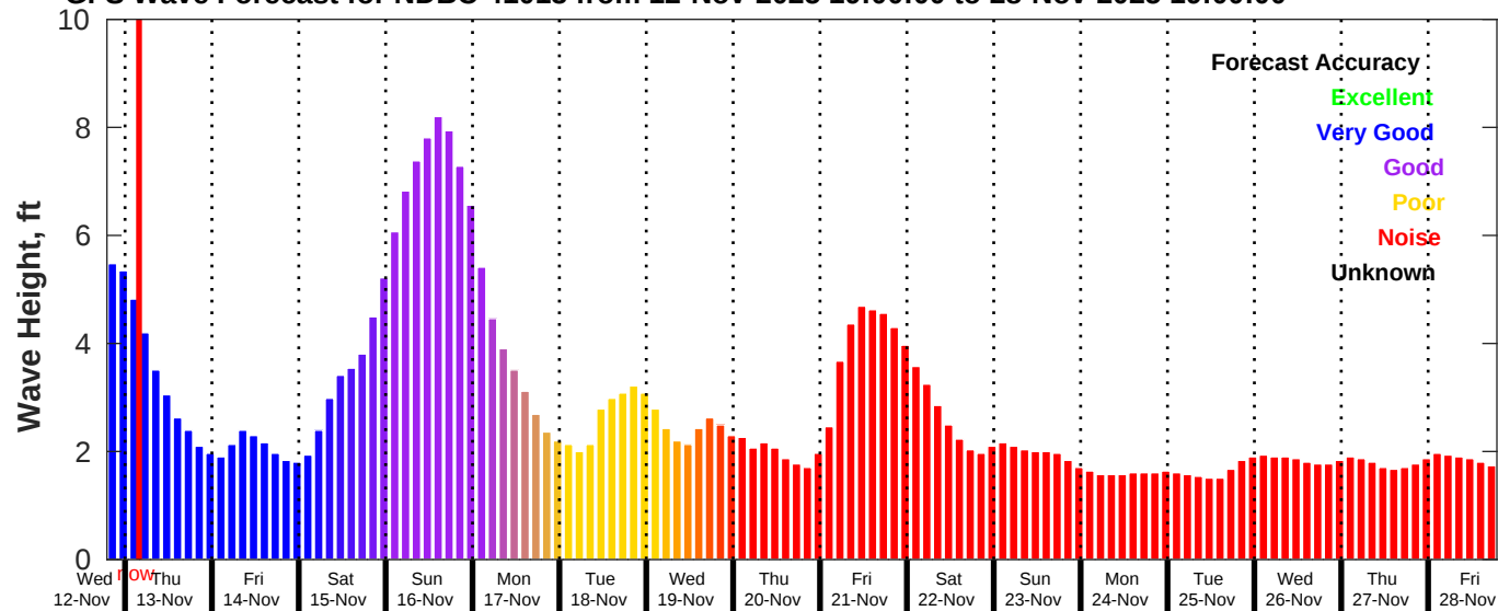
GFS Wave Forecast for NDBC 41013 from 12-Nov-2025 19:00:00 to 28-Nov-2025 19:00:00
