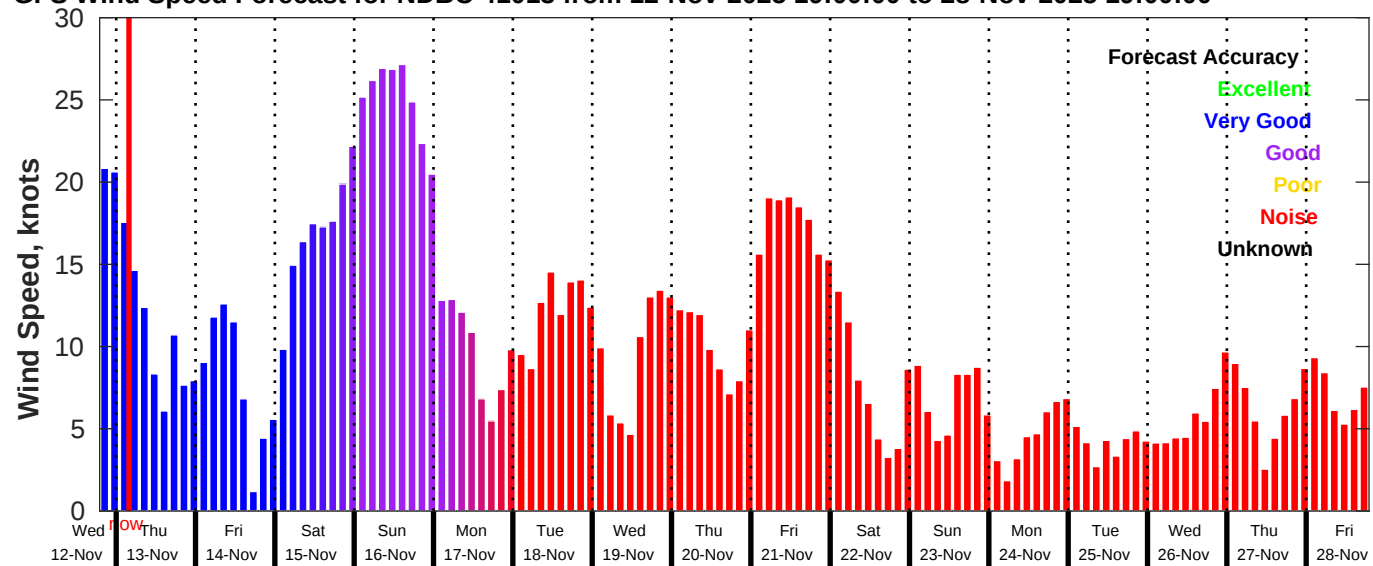
GFS Wind Speed Forecast for NDBC 41013 from 12-Nov-2025 19:00:00 to 28-Nov-2025 19:00:00
