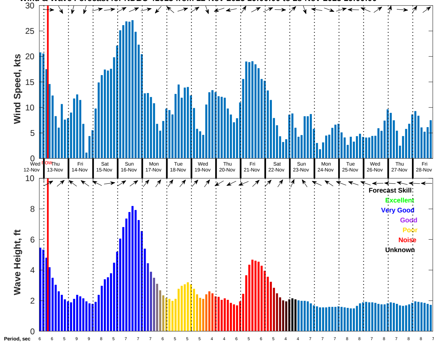
Wind & Wave Forecast for NDBC 41013 from 12-Nov-2025 19:00:00 to 28-Nov-2025 19:00:00
