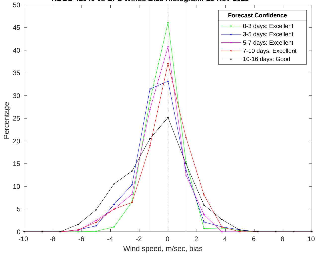
NDBC 41040 vs GFS Winds Bias Histogram: 13-Nov-2025
