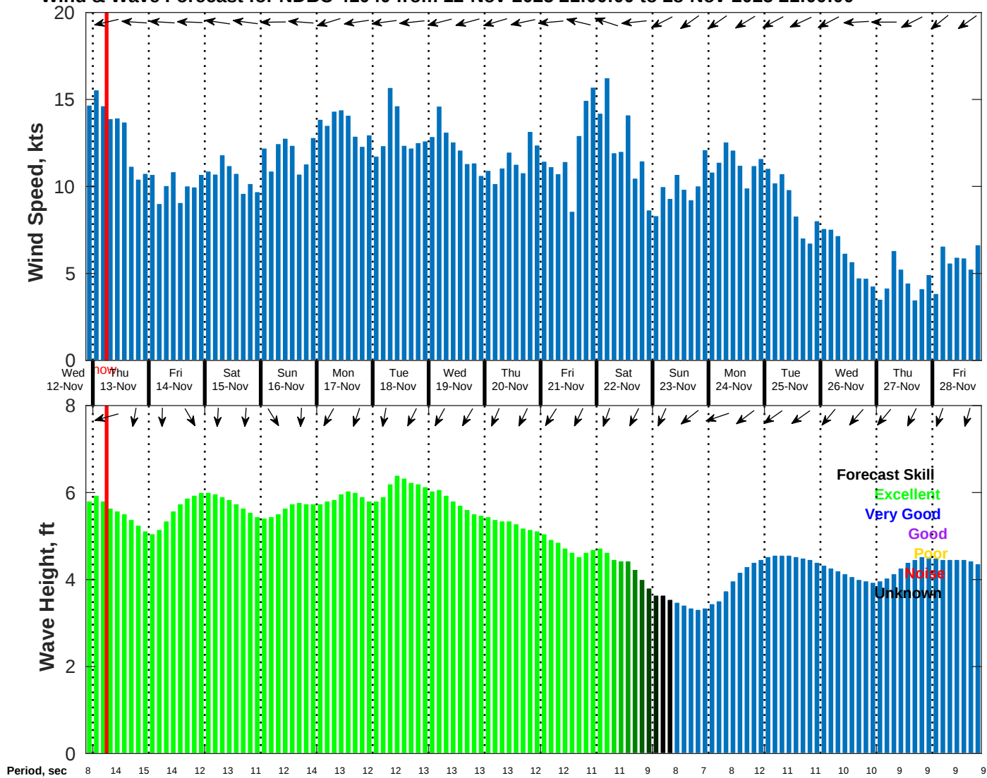
Wind & Wave Forecast for NDBC 41040 from 12-Nov-2025 21:00:00 to 28-Nov-2025 21:00:00
